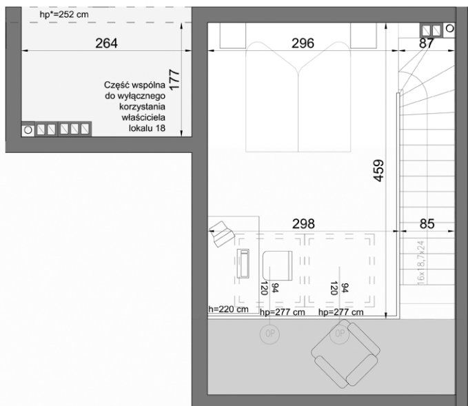
ANTRESOLA
